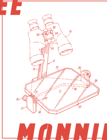
Fig. Binocular stand for astronomical observations Doehlin, Thomas A. — US Patent 4,278,320
